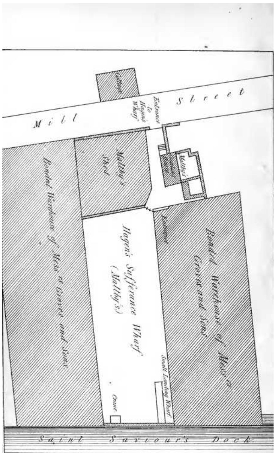
GROUND PLAN OF HAGEN'S WHARF.
